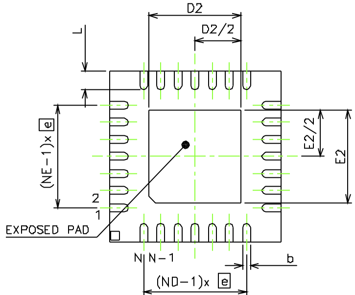
BOTTOM VIEW
